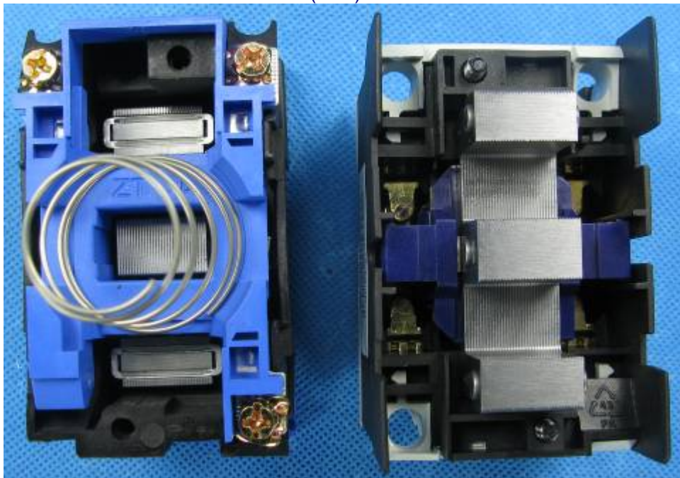
NC1-0908 (2NO+2NC) internal view
