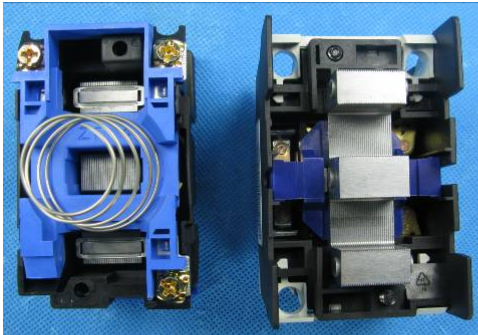
NC1-1801 internal view
