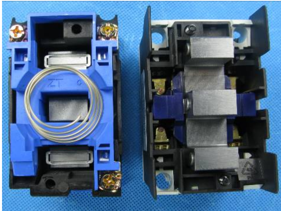
NC1-0904 (4NO) internal view
